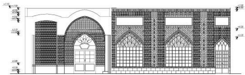
SECTION C_C
